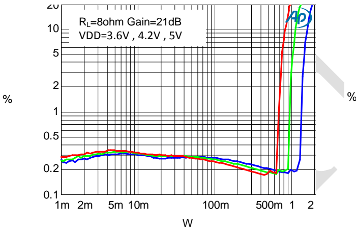
THD+N VS vs Output Power
